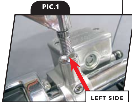
LEFT SIDE MIRROR ASSEMBLY
